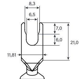
Multi-Spade Dimensions (mm)
