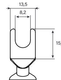
U-Spade Dimensions (mm)
