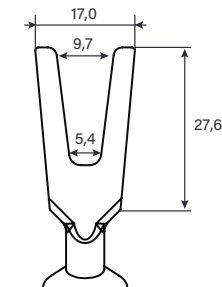
V-Spade Dimensions (mm)
